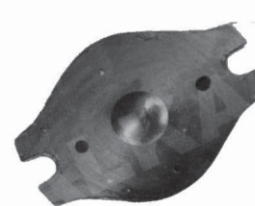
V6 80mm KSB (H) Bearing 80 x 26 x 93 x 117
