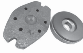
V/6 KSB 80 mm (New Model) Bearing : 80 x 25 x 97 x 118 Plate : 80 x 20 x 11 x 18 (5 x 2.5) TARBO
