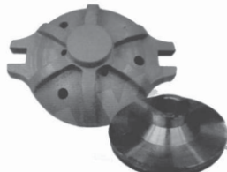
V/8 130 mm KSB SET Bearing : 130 x 68 x 130 x 160 Plate : 130 x 28 x 40 x 43 (8x3.5)
