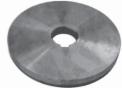
V/8 120 mm AROMA SET Plate : 1200 x 25/28 x 12.5 x 15.5 (8x3.5)
